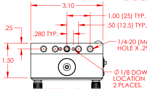
BOTTOM VIEW OF BASE
