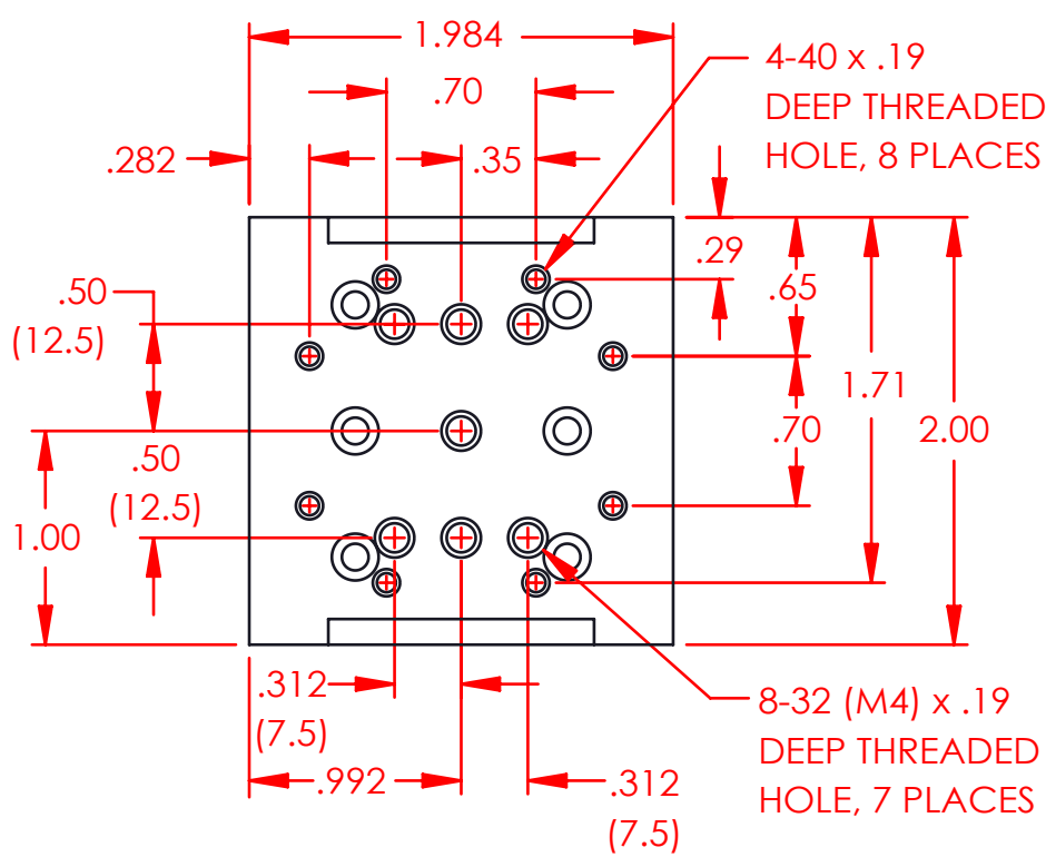
TOP PLATE
