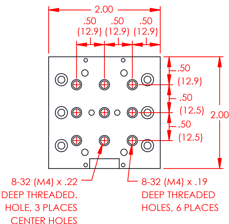
BASE PLATE
